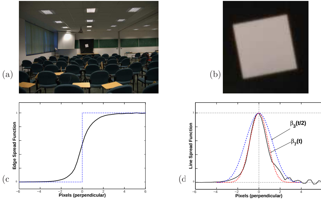
Figure 5.15: Estimation of the PSF with the slanted Edge Method; (a) Image of a slanted white square with step edges for Point Spread Function estimation (acquired with a Nikon D70s digital camera); (b) Zoom on the target; (c) Measured Edge Spread Function (solid line) and ideal step edge (dashed line); (d) Measured Line Spread Function (solid line). Its support has length 8 ranging from -4 to 4. The sampling kernel \varphi(t) can be modeled for example by either a centered B-spline of degree 7, \beta_7(t) (dashed line) or a centered B-spline of degree 3 scaled by 2, \beta_3(t/2) (dash-dot line). In both case, the sampling kernel has support 8.
