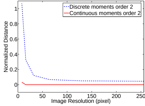
Figure 4.2: Effects of the change of resolution in the estimation of image moments of order 2. Dashed lines represent the normalized distances between the real moments and the discrete moments obtained from Equation (4.4). Solid lines represent the normalized distances between the real moments and the continuous moments obtained from Equation (4.5). As the resolution decreases, the discrete moments diverge whereas the continuous moments remain very accurate, even in the presence of noise. Similar observations are made for higher order moments.
