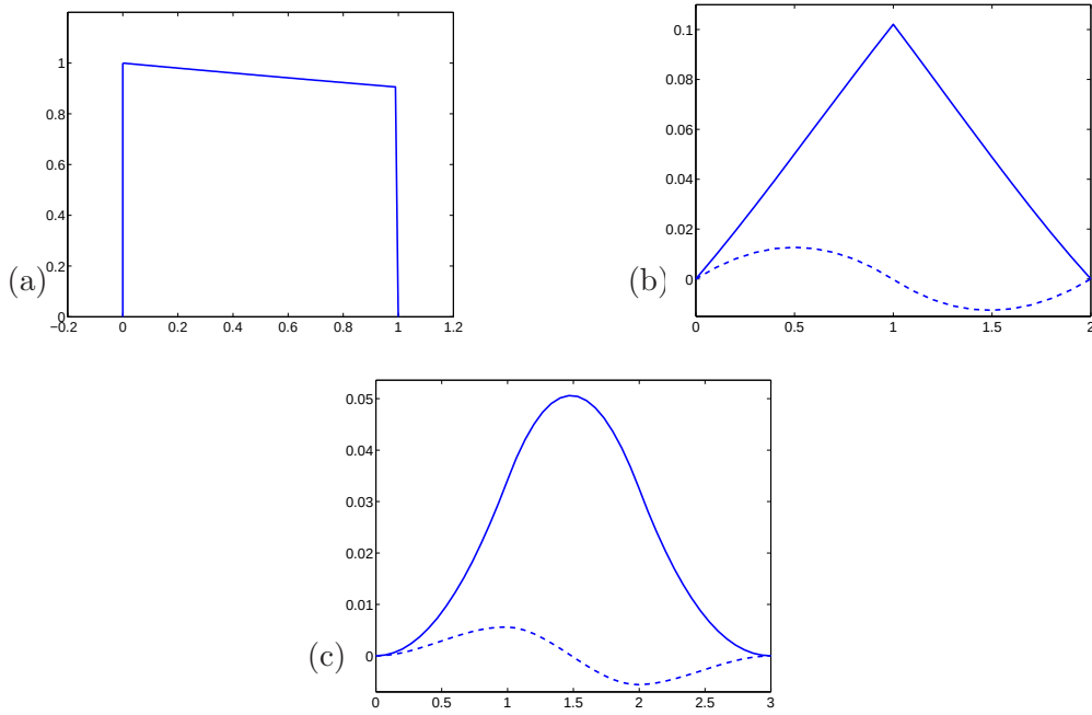
Figure 2.12: (a) Real E-spline of order 0 and parameter \alpha_0 = -0.1 ; (b) Complex E-spline of order 1 with parameters \alpha_0 = -0.05 - 0.5j , \alpha_1 = -0.5j ; (c) Complex E-spline of order 2 obtained by convolution of the two previous E-splines ( \alpha_0 = -0.05 - 0.5j , \alpha_1 = -0.5j , \alpha_2 = -0.1 ). The solid line corresponds to the real part and the dashed line to the imaginary part.
