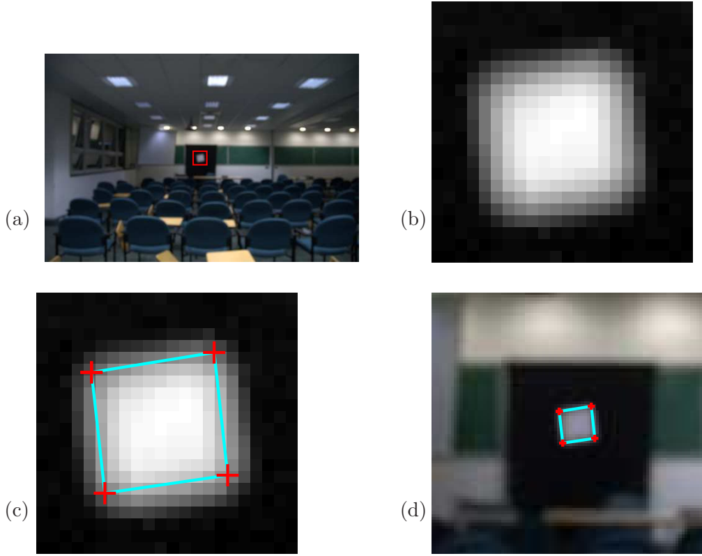
Figure 3.4: Experiment of reconstruction of a rectangle from real data. (a) Considered image of size 335x506 px resulting from a decimation by T = 6 of a blurred image taken out of focus. The square framed area is the region of interest of size 22x22 px; (b) Region of interest containing the samples of the rectangle; (c) Retrieved corners (+) and boundaries of the reconstructed rectangle. The sampling kernel is modeled by a B-spline with P = 5 and T = 6 ; (d) Retrieved rectangle in the considered image.
