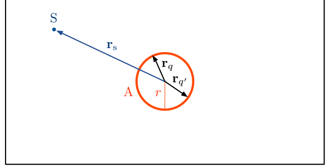
Fig. 1. Room layout in two dimensions (third dimension is not shown), showing a source S and a spherical microphone array A . Two sample microphones are located at \mathbf{r}_q = (r, \Omega_q) and \mathbf{r}_{q'} = (r, \Omega_{q'}) , and a source is located at \mathbf{r}_s = (r_s, \Omega_s) .
