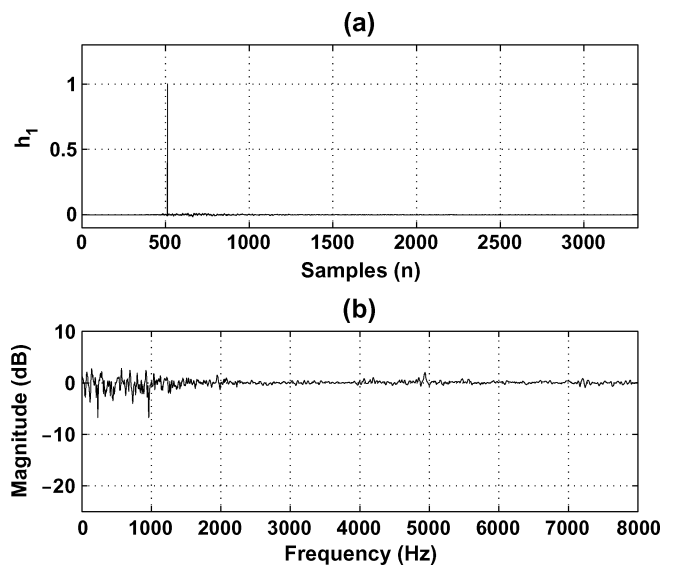
Fig. 13. Equalized (a) time-domain impulse response and (b) magnitude response, using the SB-MCEQ method for \mathcal{M}_m = -50 dB.
