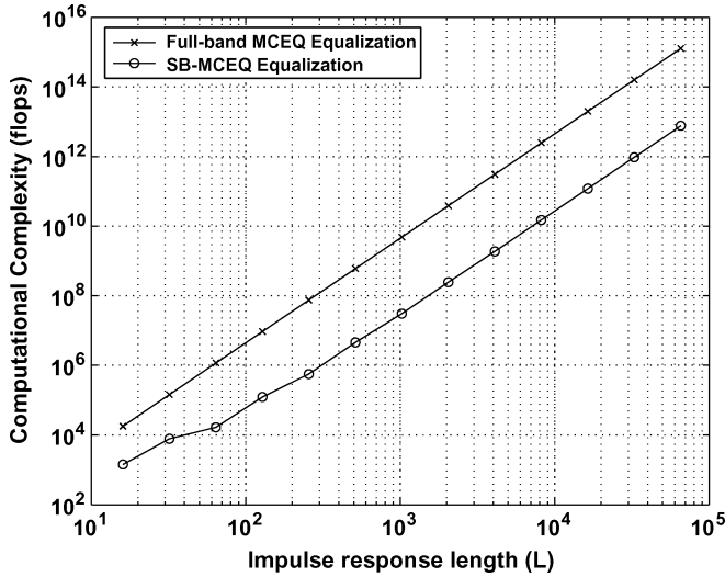
Fig. 5. Floating point operation count versus system length for the full-band (x) and subband (o) equalizers.
