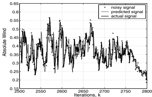
Fig. 3. Prediction performance for complex wind signal using ACEKF
