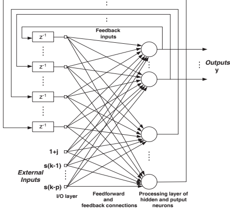
Fig. 1. A fully connected recurrent neural network (FCRNN) for prediction.
