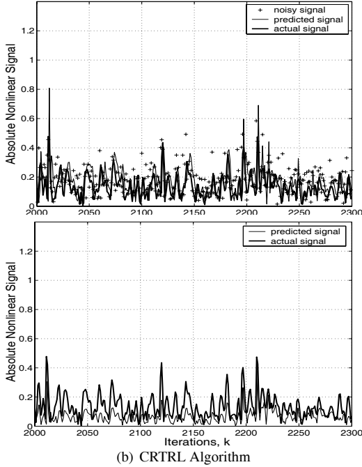
Fig. 2. Comparison of one-step ahead prediction performance between the ACEKF and CRTRL for nonlinear signal (19)
