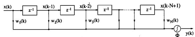
Fig. 1. Nonlinear neural adaptive filter.
