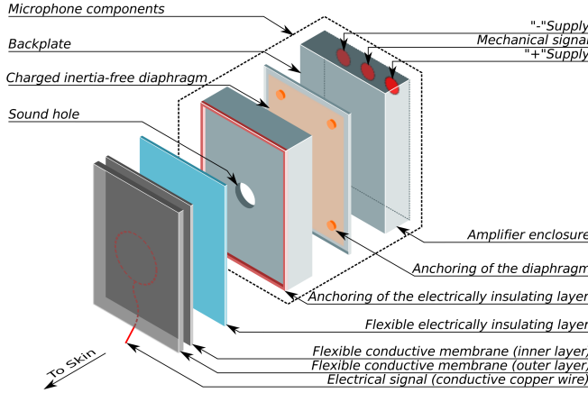
Fig. 1. Detailed construction diagram of the multimodal sensor.
