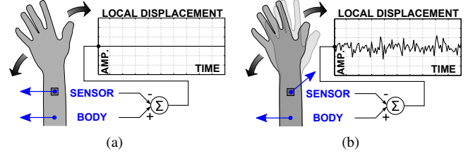
Fig. 2. Principle of the multimodal sensor. (a) The diaphragm inside the mechanical transducer has very small mass, thus body movements which do not cause displacements of the electrode with respect to skin are not detected. (b) Abrupt movements leading to displacements of the sensor with respect to the skin are detected by the mechanical transducer directly through the surface; such a mechanical signal can be used to denoise the electrical signal.
