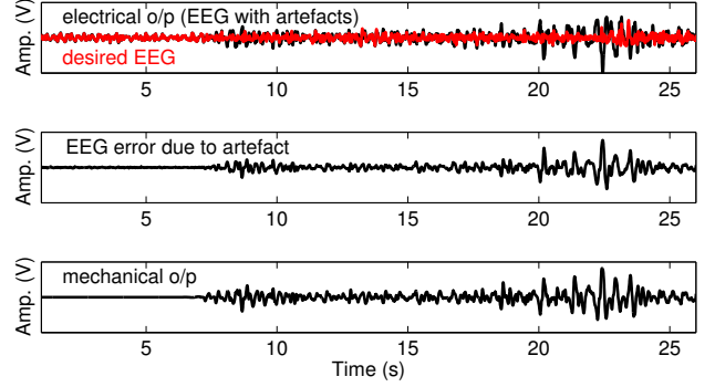
Fig. 4. Motion artefact detection. Top panel: the EEG signal corrupted with motion artefact together with the clean EEG obtained by averaging the signals from four standard electrodes. Middle panel: the difference between the noisy and clean EEG signal. Lower panel: the mechanical output of the multimodal sensor.
