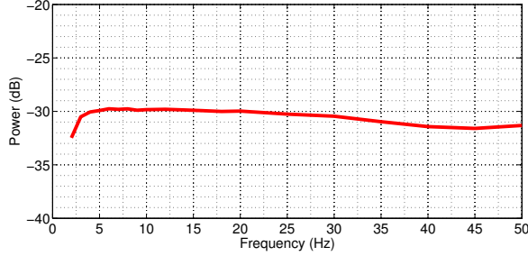
Fig. 3. Frequency response of the mechanical part of the multimodal sensor. The sensor was firmly attached to the vibration plate oscillating at a 1 mm displacement amplitude and the frequency was varied over a 2 – 50Hz range.
