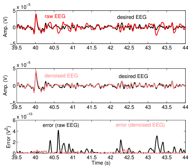
Fig. 5. Motion artefact removal. Top panel: clean/desired and corrupted EEG signals. Middle panel: desired and denoised EEG signals. Lower panel: the squared error prior to and after denoising.
