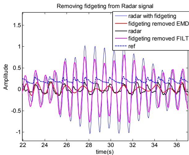
Fig. 6 Removing the fidgiting interference using both EMD and filtering. Emphasizing the fact that only filtering cannot remove this type of interference while EMD is effective.
