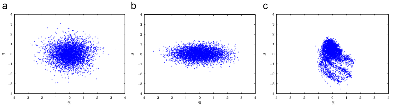
Fig. 1. Distributions of an AR(4) process for different realisations of the driving noise. (a) AR(4) driven by circular noise. (b) AR(4) driven by doubly white noncircular noise. (c) AR(4) driven by general noncircular noise.
