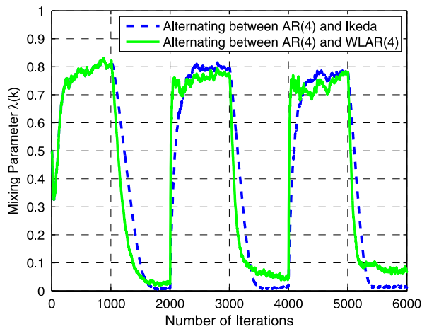
Fig. 7. Evolution of the mixing parameter \lambda for signals alternating from linear AR(4) to either widely linear AR(4) model of the Ikeda process or the original Ikeda signal.
