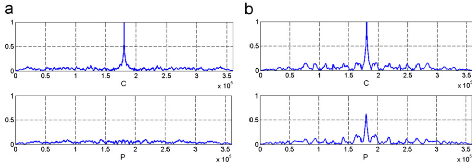
Fig. 11. Normalised covariance (top) and pseudocovariance (bottom) for 1 h sections of wind data. (a) Calm wind. (b) High wind.
