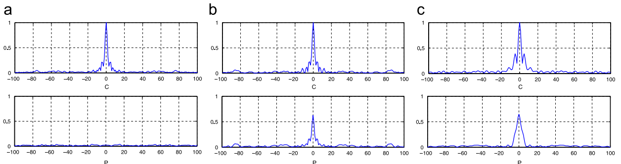
Fig. 2. Covariance (top) and pseudocovariance (bottom) of a standard AR(4) model driven by different driving noises. (a) AR(4) driven by doubly white circular noise. (b) AR(4) driven by doubly white noncircular noise. (c) AR(4) driven by general noncircular noise.
