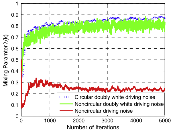
Fig. 6. Evolution of the mixing parameter \lambda for a standard linear AR(4) model driven by noises of different nature.
