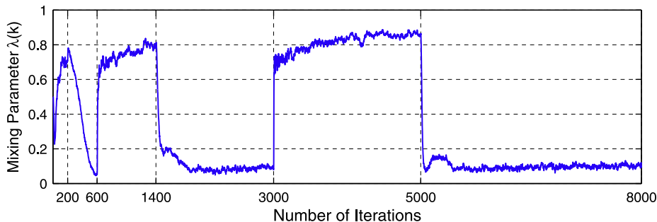
Fig. 8. Evolution of the mixing parameter \lambda for a signal alternating from a proper AR(4) to an improper linear AR(4) process with a varying segment duration.
