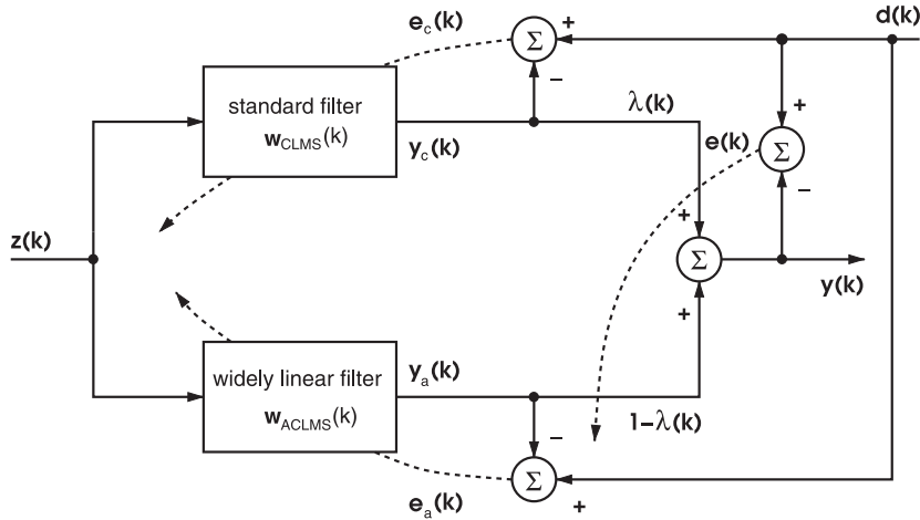
Fig. 4. Hybrid filter structure.
