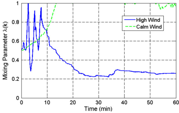
Fig. 12. Evolution of the mixing parameter \lambda(k) for 1 h of 'calm' wind and 1 h of 'high' wind.
