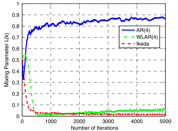
Fig. 5. Evolution of the mixing parameter \lambda for the linear circular AR(4) process, the WLAR(4) model of the Ikeda map (improper) and the original noncircular Ikeda signal.
