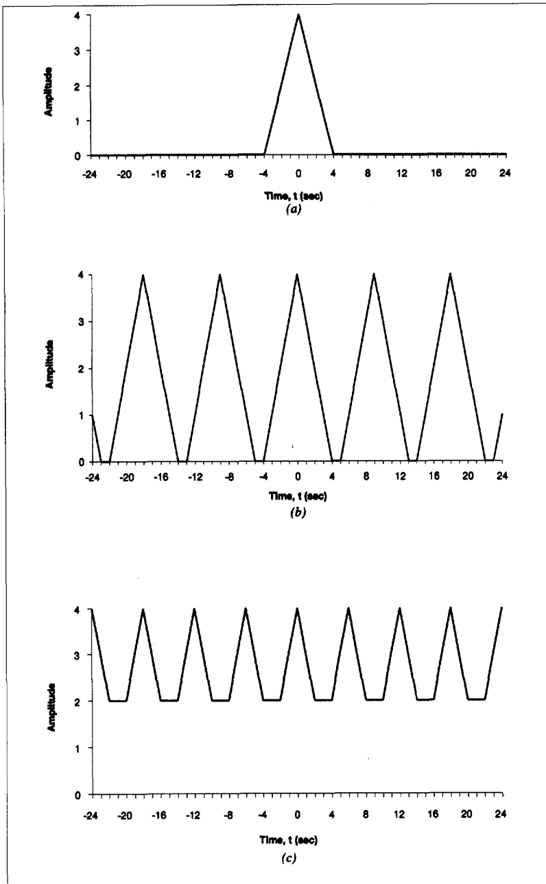
1. (a) The signal x_1(t) . The "time width" is T_1 = 8 s. (b) The signal y(t) when the period T_y = 9 is chosen greater than T_1 . (c) The signal y(t) when T_y = 6 \leq T_1 .
