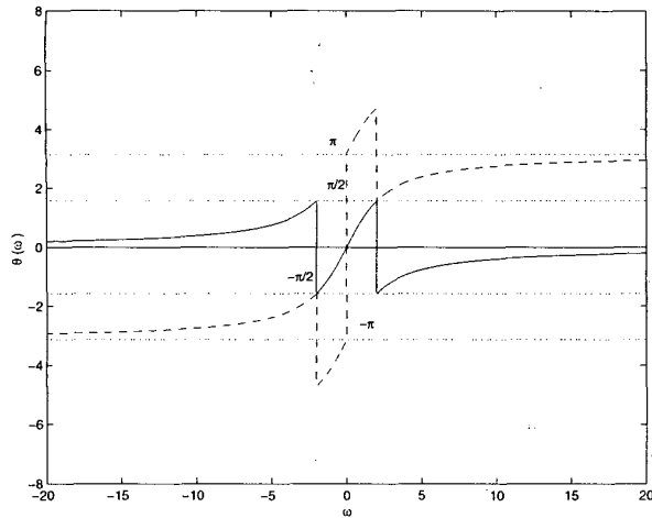
Figure 2: The exact curves from equations (6) and (8)
