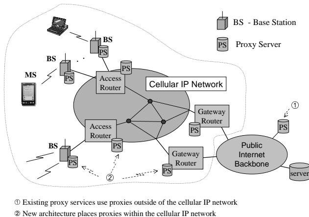
Fig. 1. General architecture of a cellular IP network with proxy servers.
