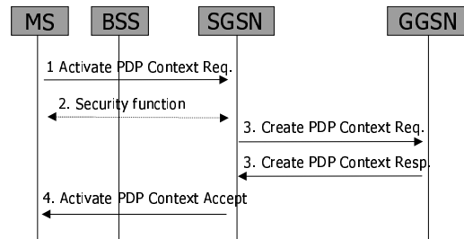
Fig. 4. PDP context activation procedure.
