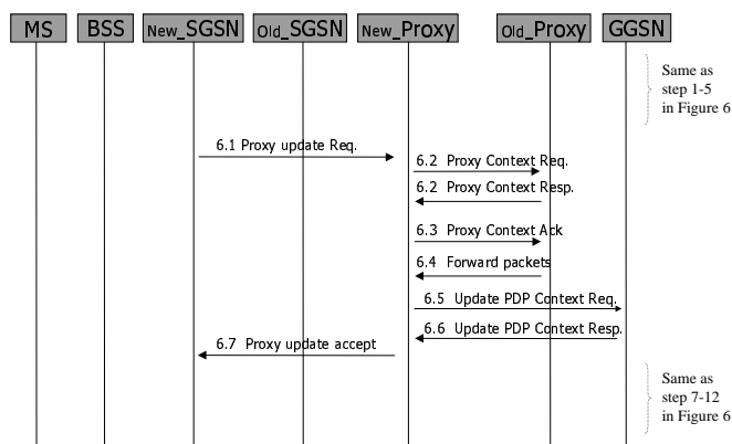
Fig. 7. GPRS mobility update procedure with proxy support.
