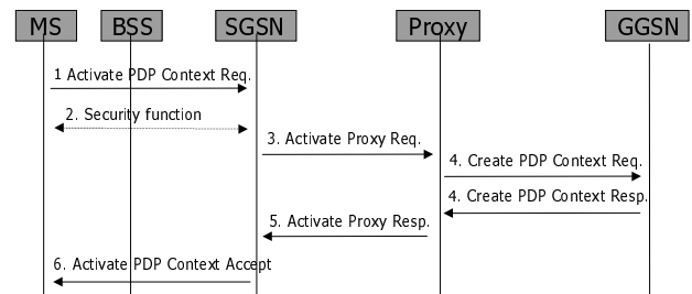
Fig. 6. PDP context activation procedure with proxy supports.
