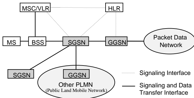
Fig. 3. GPRS Logical Architecture.
