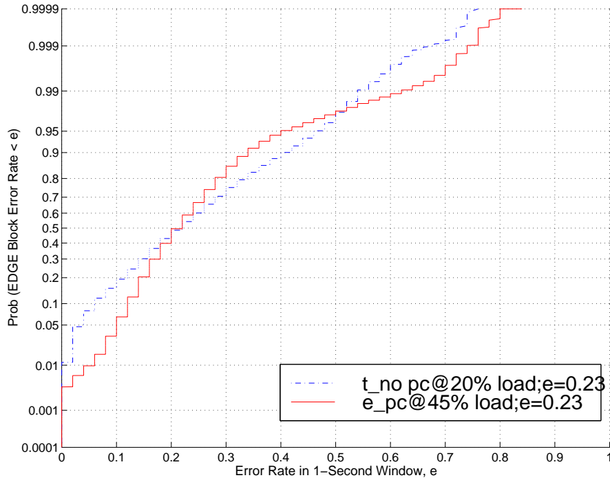
Figure 6. CDF of EDGE Block Error Rate with 20/45% Load
