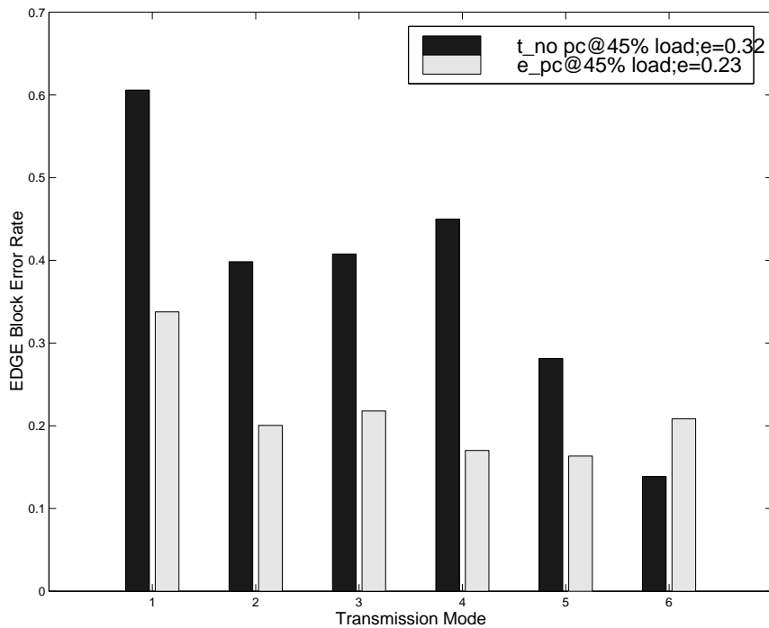
Figure 3. EDGE Block Error Rate Vs. Transmission Mode
