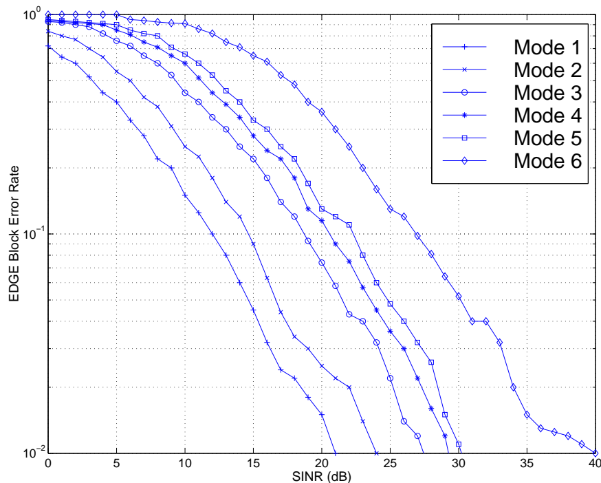
Figure 2. EDGE Block Error Rate Vs. SINR
