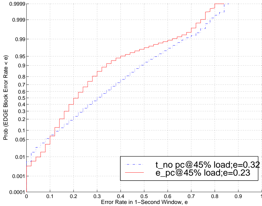
Figure 4. CDF of EDGE Block Error Rate with 45% Load
