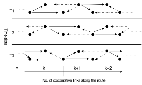
Fig. 6. TDM-schedule for a cooperative route with M=1
